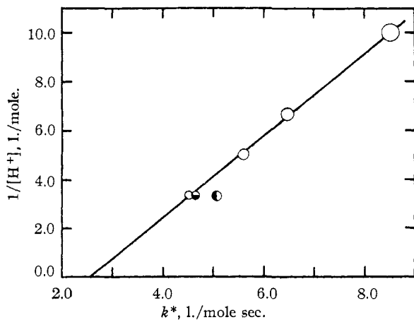
Fig. 2.—Variation of k^* with 1/[\text{H}^+] for 2,6-dibromophenol at [\text{Br}^-] equal 0.292–0.296 M (O), 0.196 M (◐), and 0.097 M (●). Points drawn with radius equal 2% of k^* .
