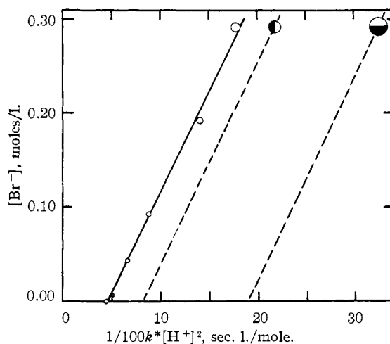
Fig. 4.— [\text{Br}^-] vs. 1/100k^*[\text{H}^+]^2 for 3,5-dibromo-2-hydroxybenzoic acid at [\text{H}^+] equal 0.300 M (O), 0.200 M (O), and 0.100 M (●).
