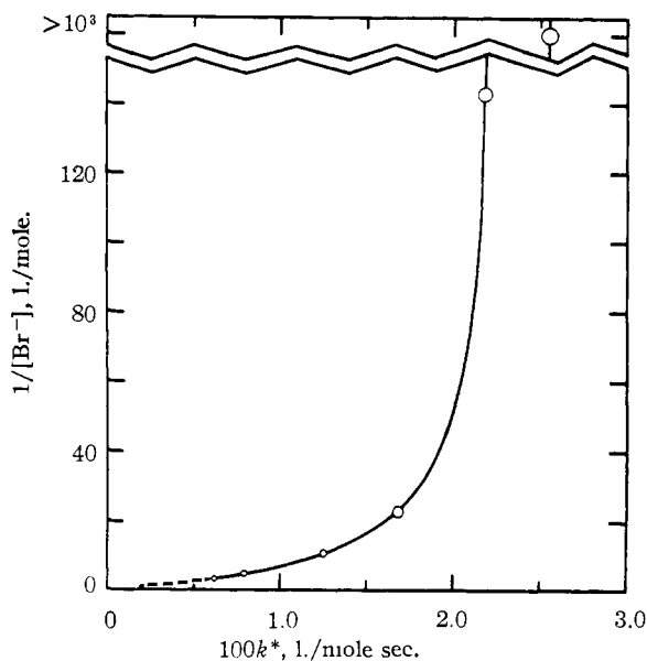
Fig. 3.—Variation of k^* with 1/[\text{Br}^-] for 3,5-dibromo-2-hydroxybenzoic acid at [\text{H}^+] = 0.300 M ; points drawn with radius equal 2% of k^* .
