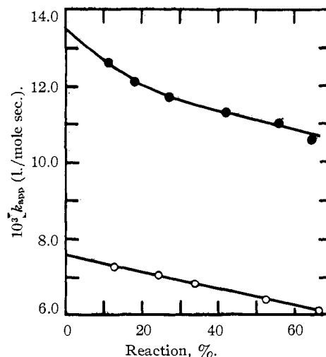
Fig. 1.—Integrated second-order rate constants vs. percentage reaction for 3,5-dibromo-2-hydroxybenzoic acid (●) in 75.0% acetic acid, (HBr) 0 = 0.0100 M , (HClO 4 ) = 0.290 M ; 3,5-dibromo-4-hydroxybenzoic acid (○) in 80.0% acetic acid, (HBr) 0 = 0.050 M , (HClO 4 ) = 0.250 M .
